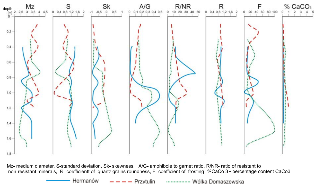
Text-fig. 6. Results of lithological analyses of sediments covering lacustrine deposits of the Mazovian Interglacial and early Livian (based on Żarski et al. 2009b).
